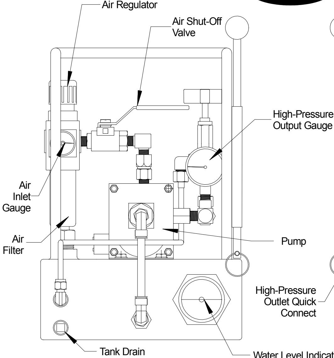
FRONT VIEW
