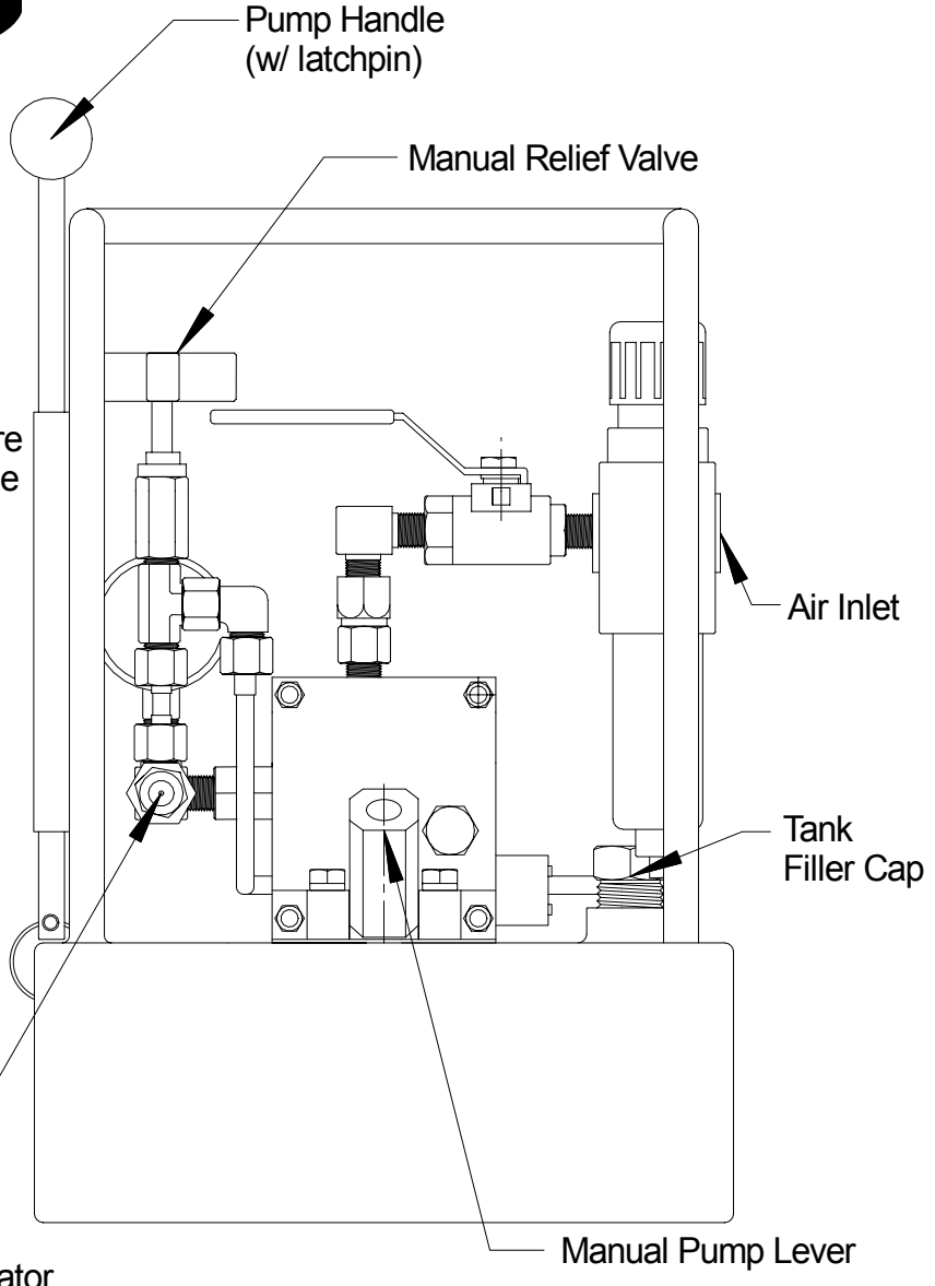
REAR VIEW
