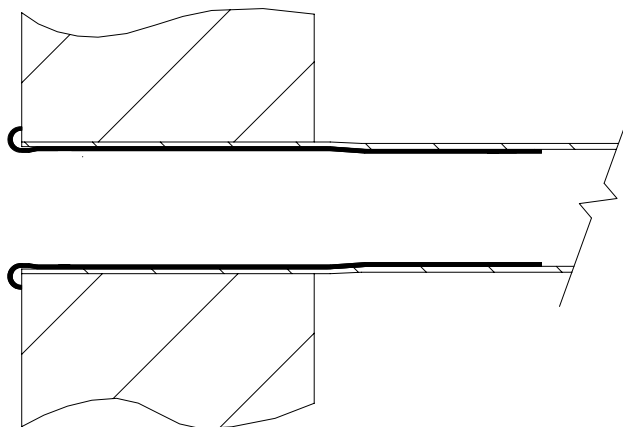
Completed SleevePro® strain controlled installation
