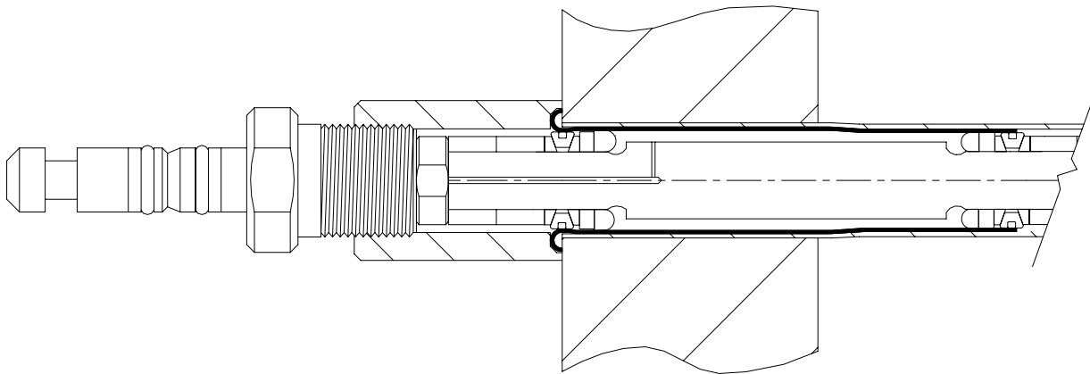
After strain controlled expansion
