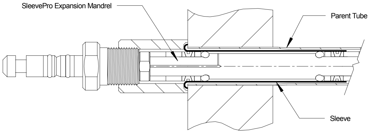
SleevePro® expansion mandrel and sleeve prior to expansion
